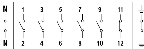
Schemat 1: GS 01 3 NO + 2 NO + 1 NC
