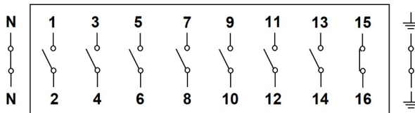
Schemat 2: GS 03 6 NO + 1 NO + 1 NC
