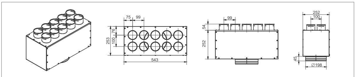
REQUBOX 10-75/200
