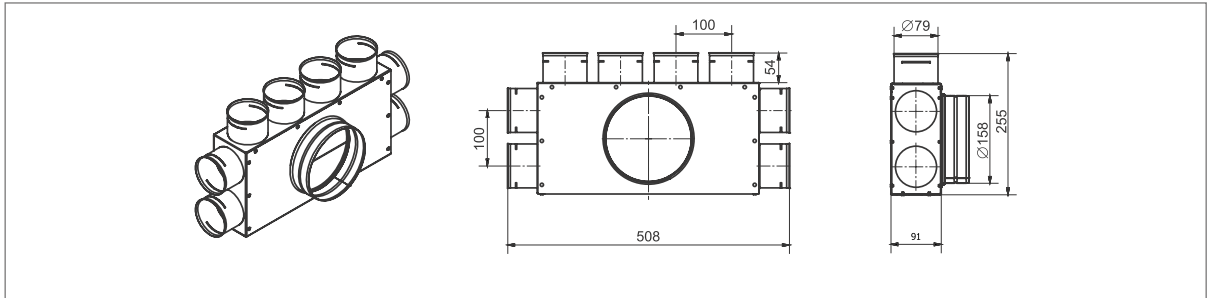
REQUBOX 8-75/160
