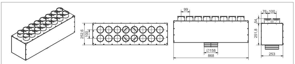
REQUBOX 16-75/160
