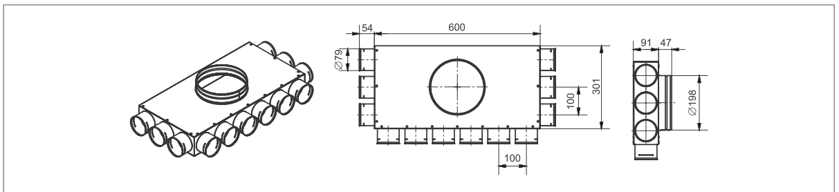
REQUBOX 12-75/200
