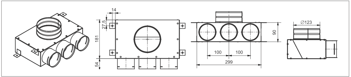
REQUBOX 3-75/125
